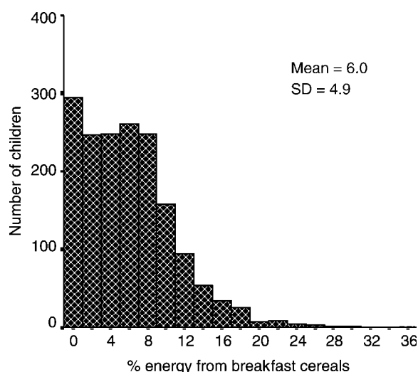
Fig. 1 Percentage of energy from breakfast cereals: distribution for all children ( n = 1688 ). SD – standard deviation
